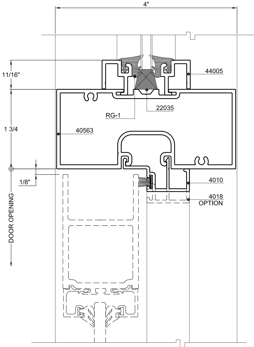
41 DOOR TRANSOM HEAD
