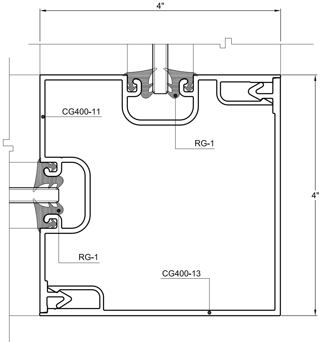
32 WIDE OUTSIDE CORNER
